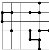
Figure 3.6: Percolation site-lien.
